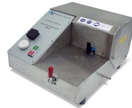
TBS-4A Automatic food Twin Blade Saw
